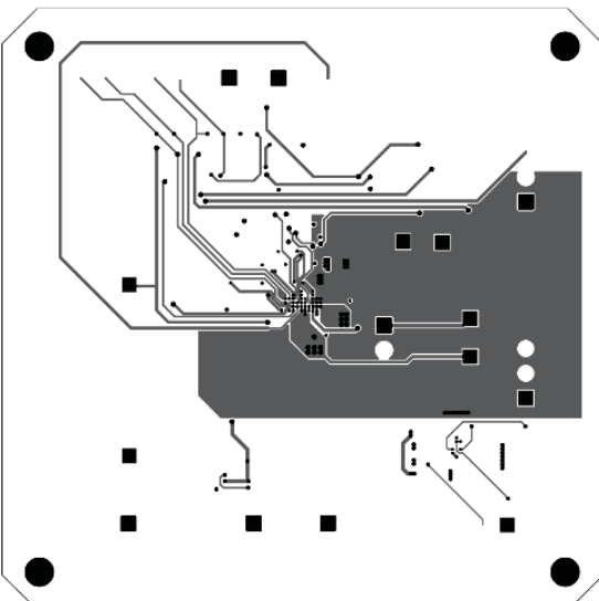
Figure 16: Mid layer 1
