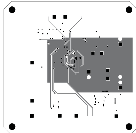
Figure 17: Mid layer 2
