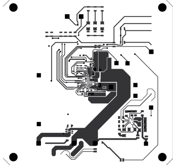
Figure 15: Top layer
